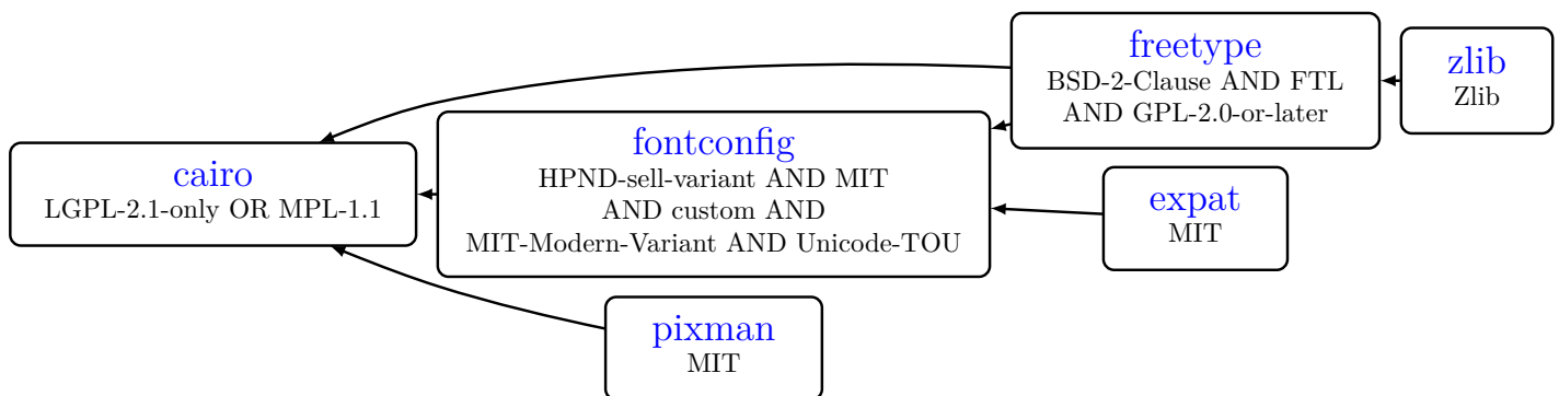
Figure 12.1: Dependency tree for cairo
