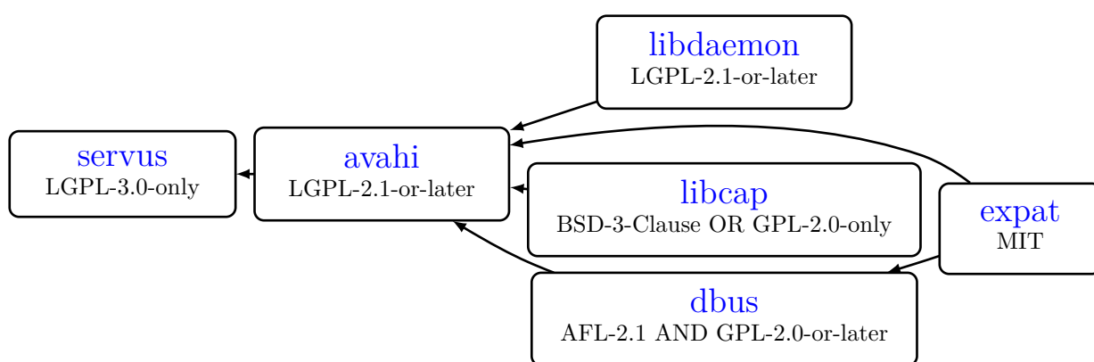
Figure 116.1: Dependency tree for servus
