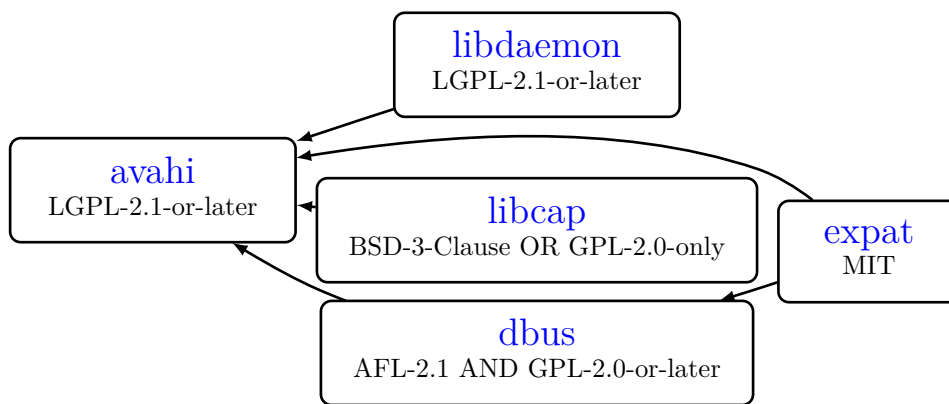
Figure 5.1: Dependency tree for avahi
