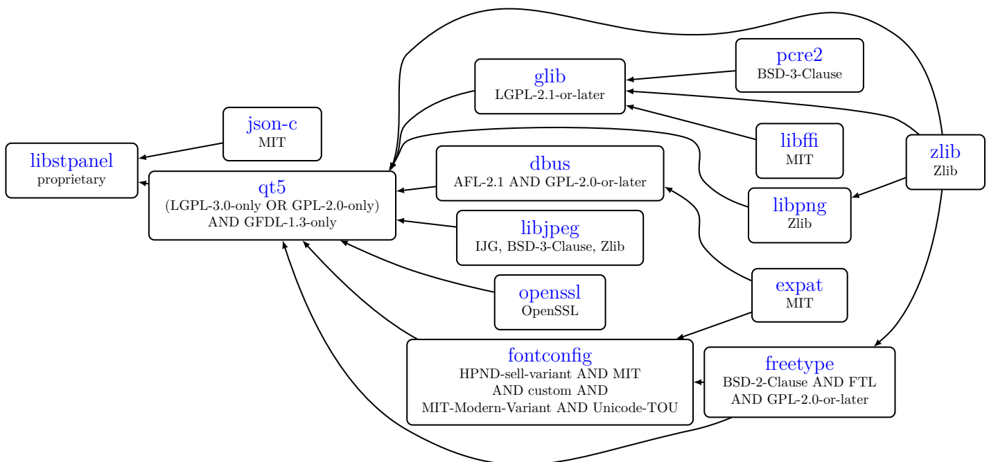
Figure 76.1: Dependency tree for libstpanel
