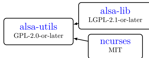
Figure 2.1: Dependency tree for alsa-utils
