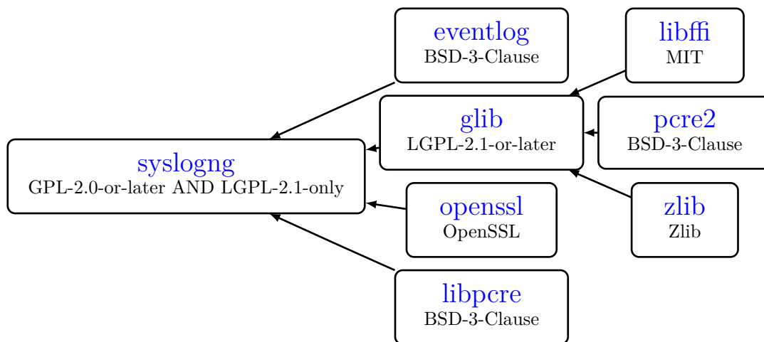
Figure 121.1: Dependency tree for syslogng
