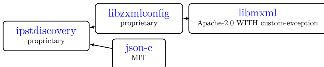
Figure 40.1: Dependency tree for ipstdiscovery
