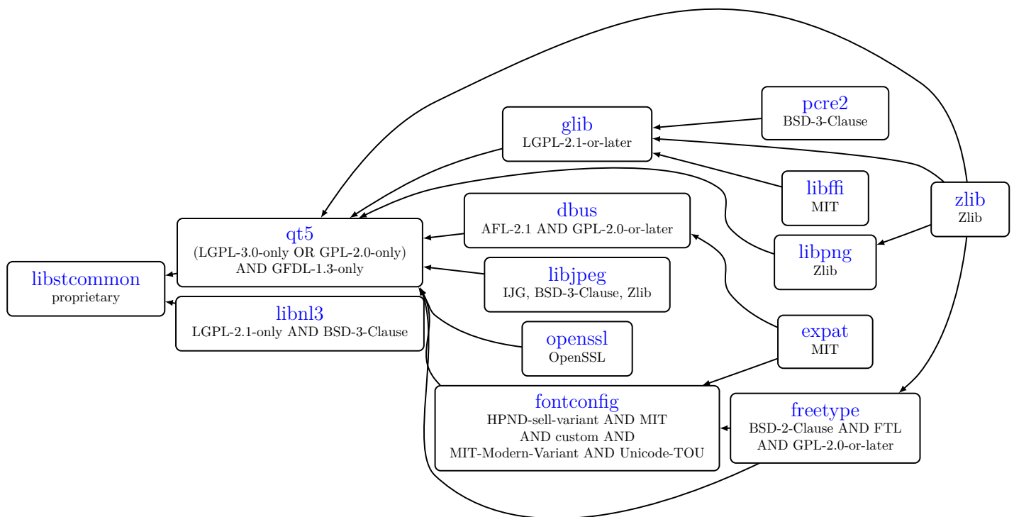
Figure 75.1: Dependency tree for libstcommon
