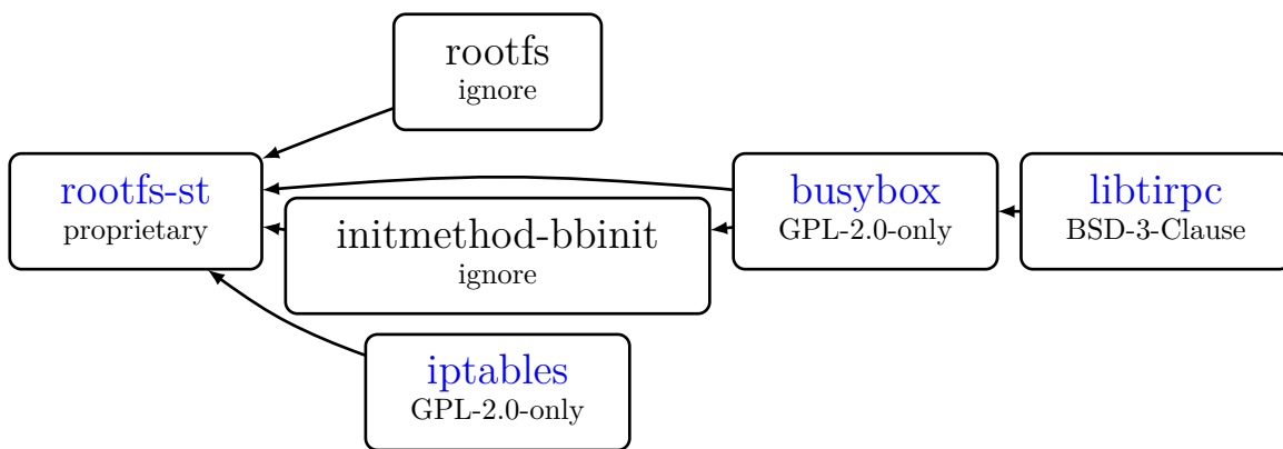
Figure 115.1: Dependency tree for rootfs-st
