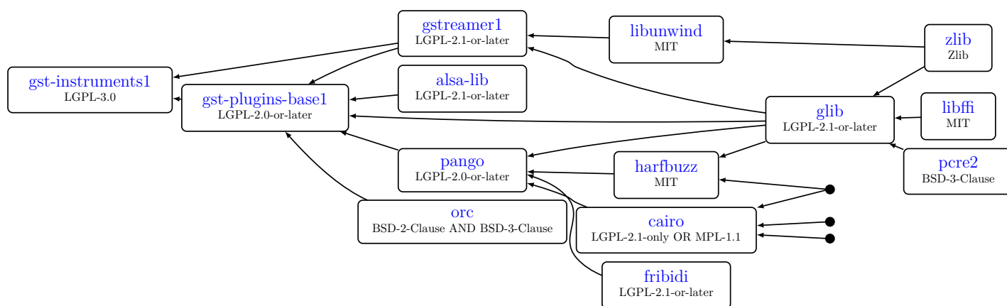
Figure 29.1: Dependency tree for gst-instruments1
