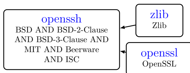
Figure 101.1: Dependency tree for openssh
