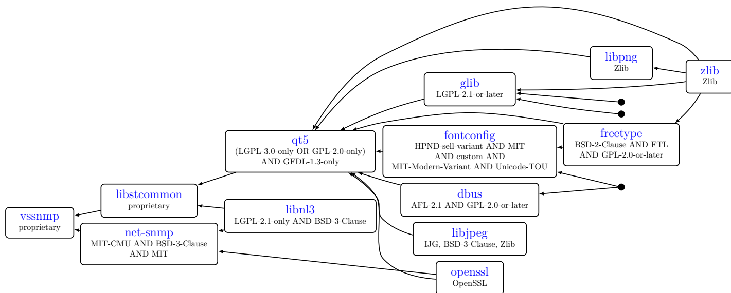
Figure 130.1: Dependency tree for vssnmp
