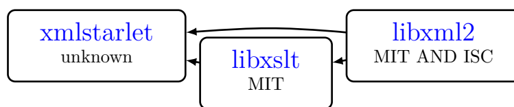
Figure 138.1: Dependency tree for xmlstarlet
