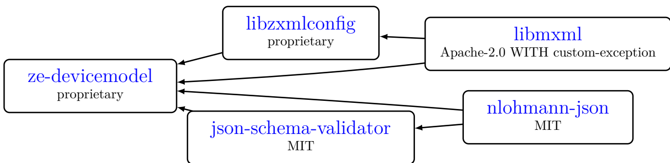
Figure 145.1: Dependency tree for ze-devicemodel
