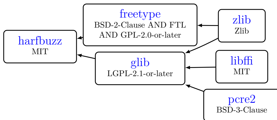
Figure 35.1: Dependency tree for harfbuzz
