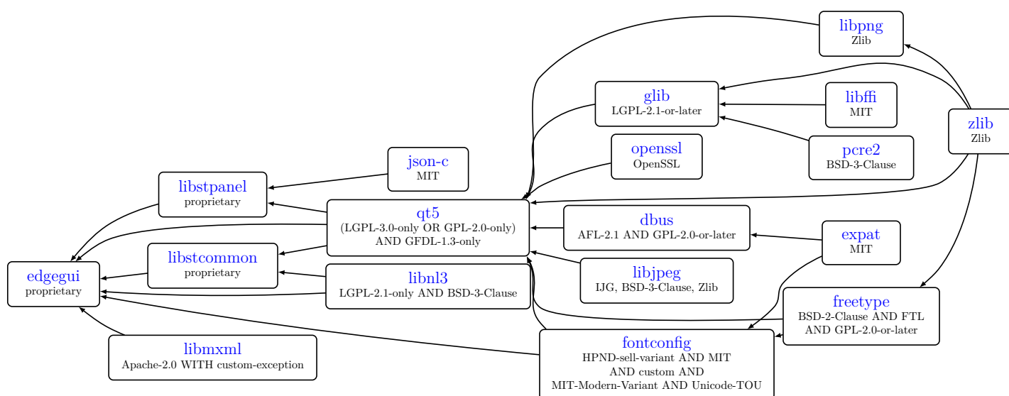
Figure 17.1: Dependency tree for edgegui
