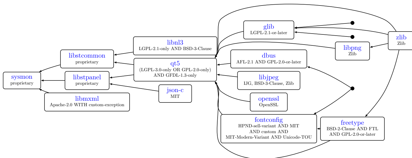
Figure 122.1: Dependency tree for sysmon
