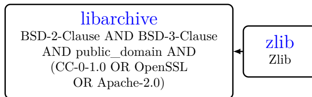
Figure 47.1: Dependency tree for libarchive
