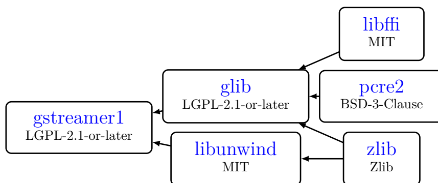
Figure 34.1: Dependency tree for gstreamer1
