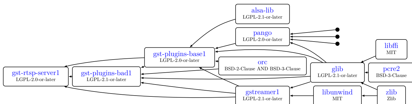
Figure 33.1: Dependency tree for gst-rtsp-server1
