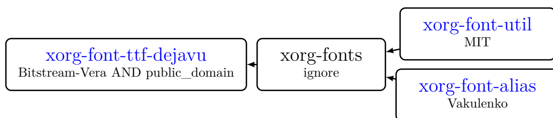
Figure 142.1: Dependency tree for xorg-font-ttf-dejavu
