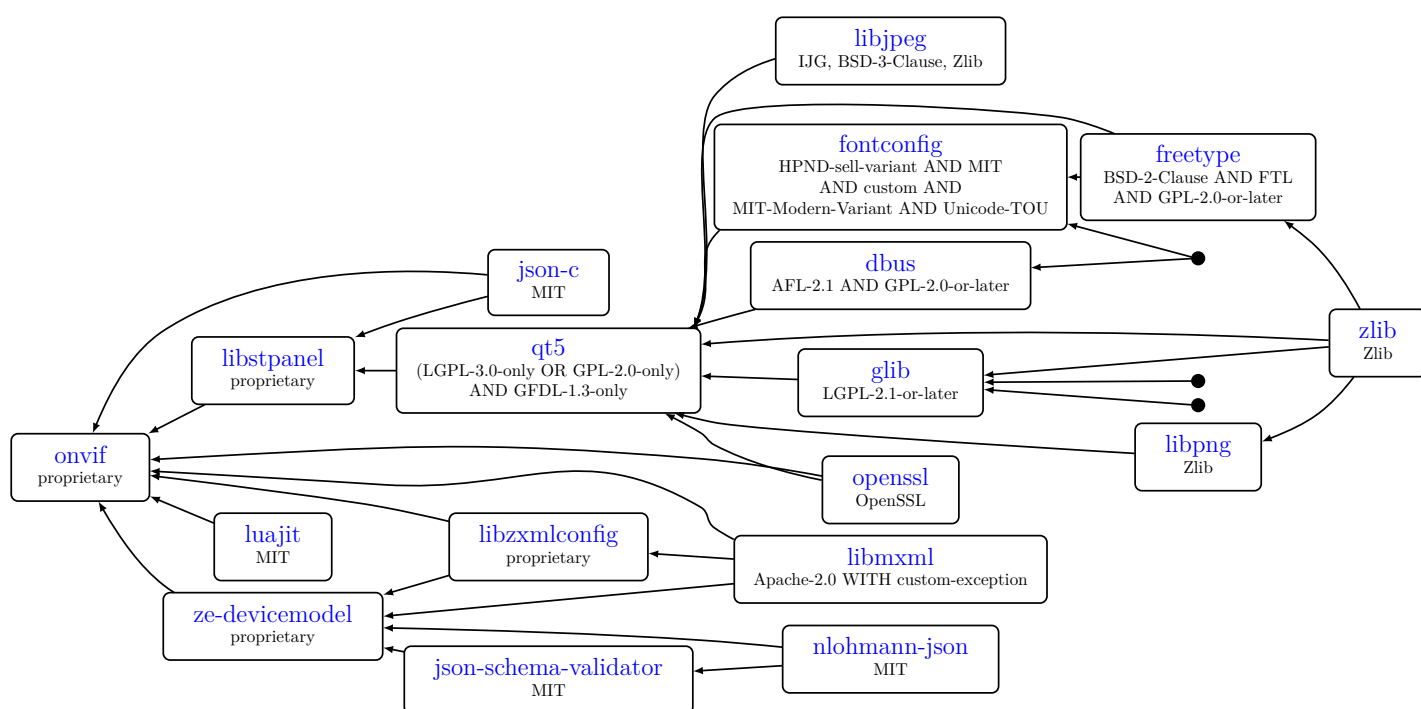
Figure 100.1: Dependency tree for onvif
