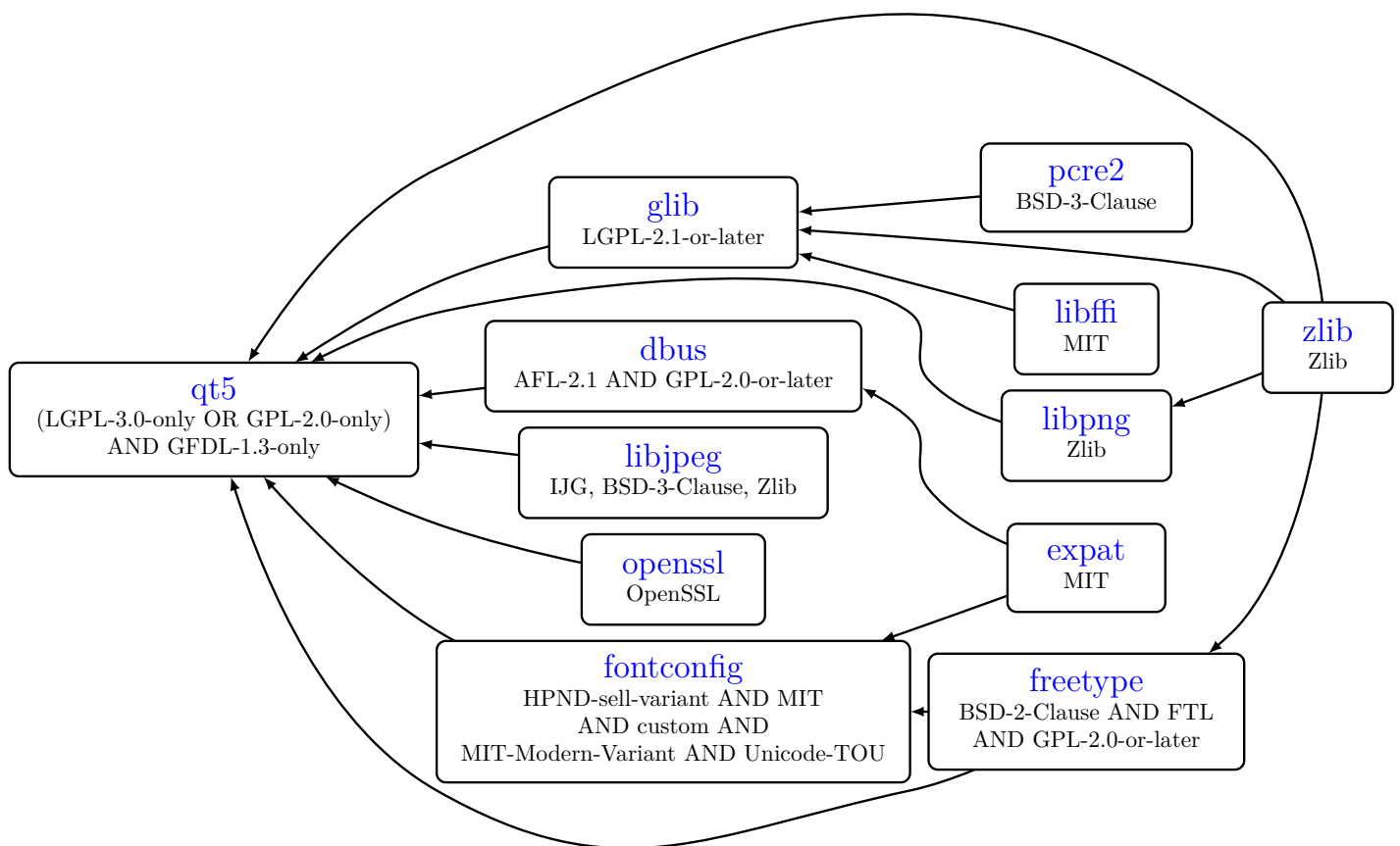
Figure 113.1: Dependency tree for qt5
