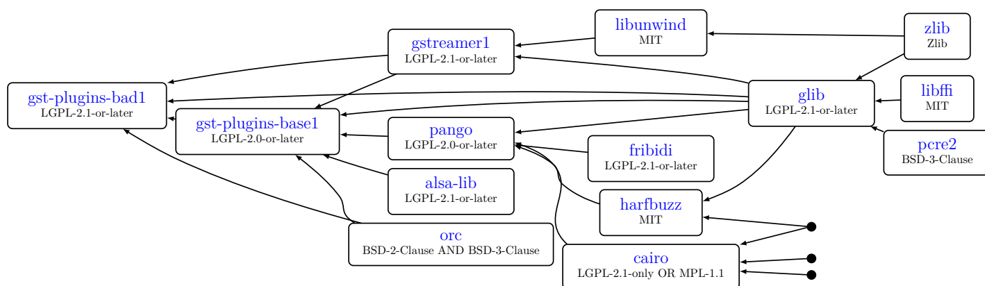
Figure 30.1: Dependency tree for gst-plugins-bad1
