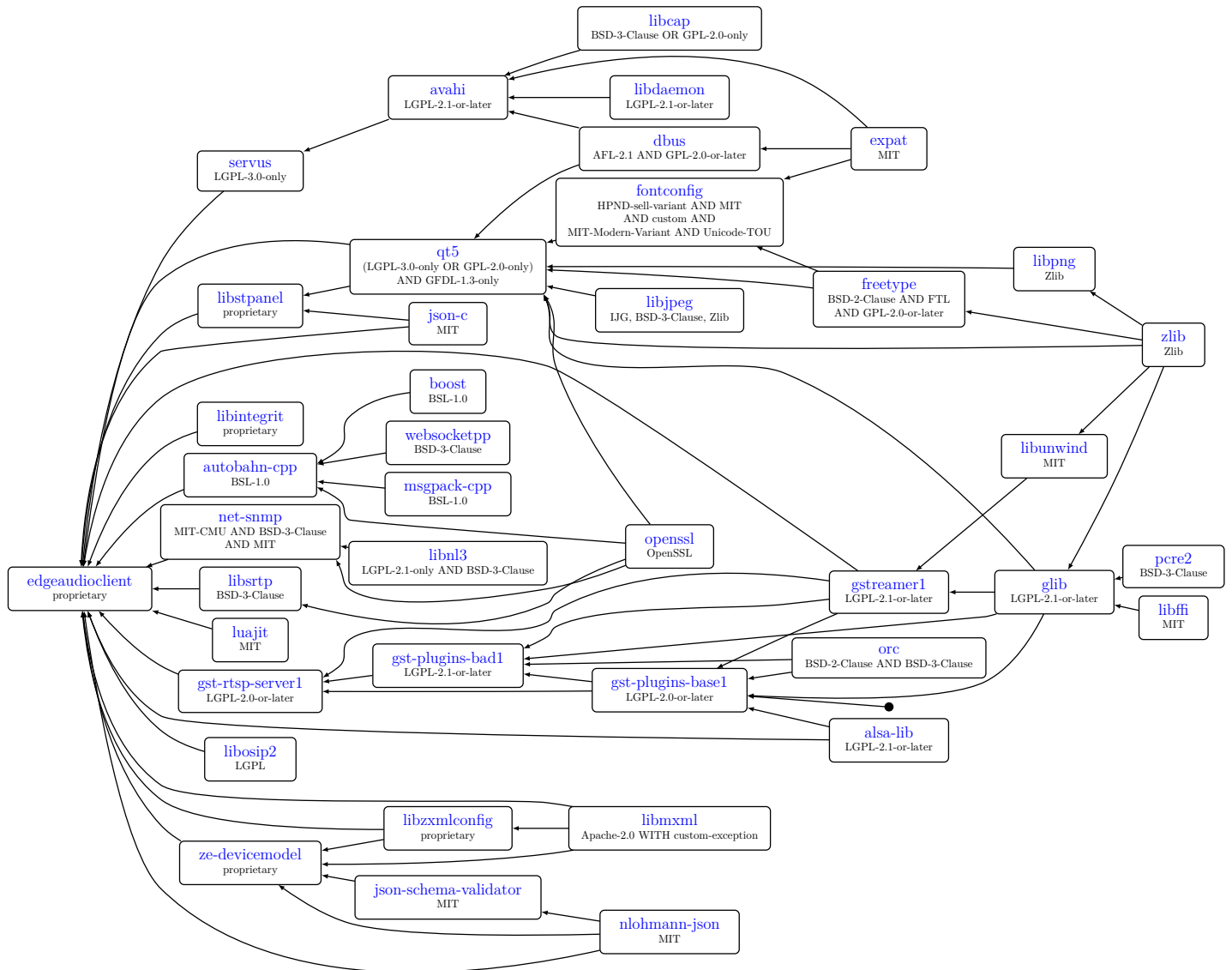
Figure 16.1: Dependency tree for edgeaudioclient
