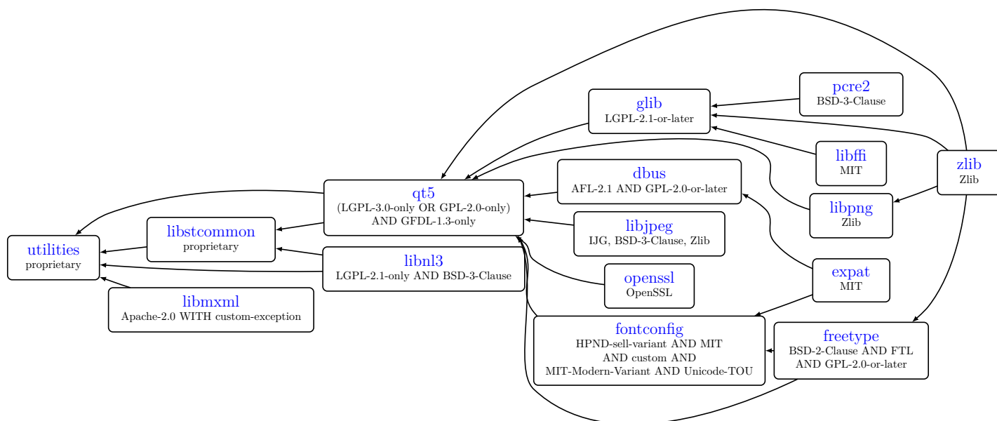
Figure 129.1: Dependency tree for utilities
