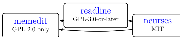
Figure 88.1: Dependency tree for memedit
