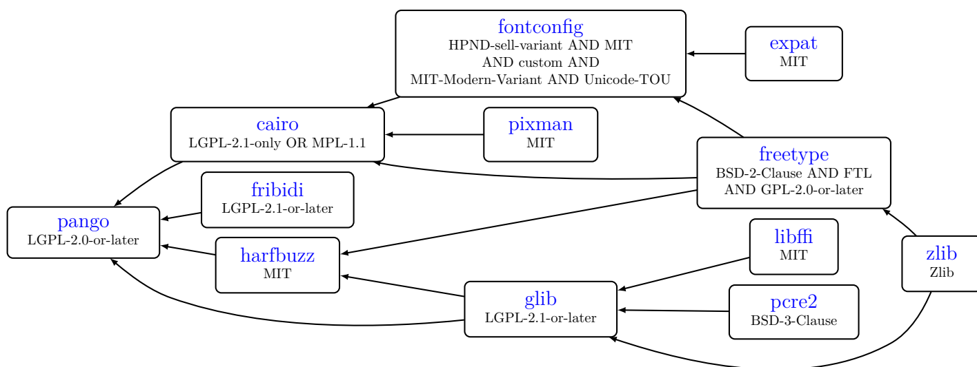
Figure 108.1: Dependency tree for pango
