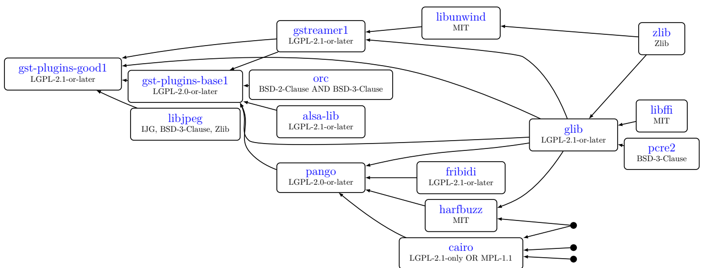
Figure 32.1: Dependency tree for gst-plugins-good1
