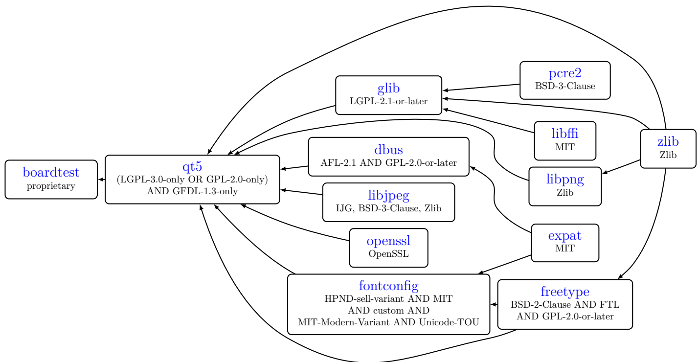
Figure 7.1: Dependency tree for boardtest
