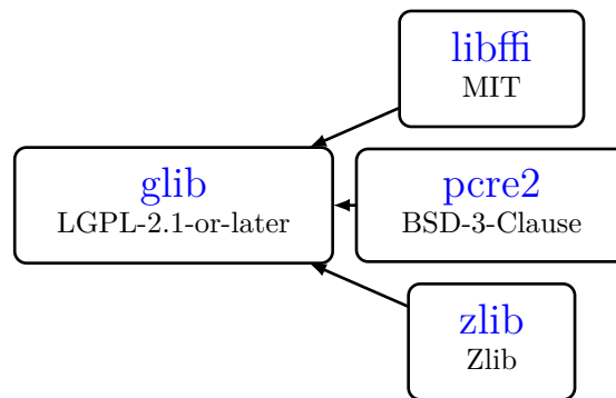
Figure 27.1: Dependency tree for glib
