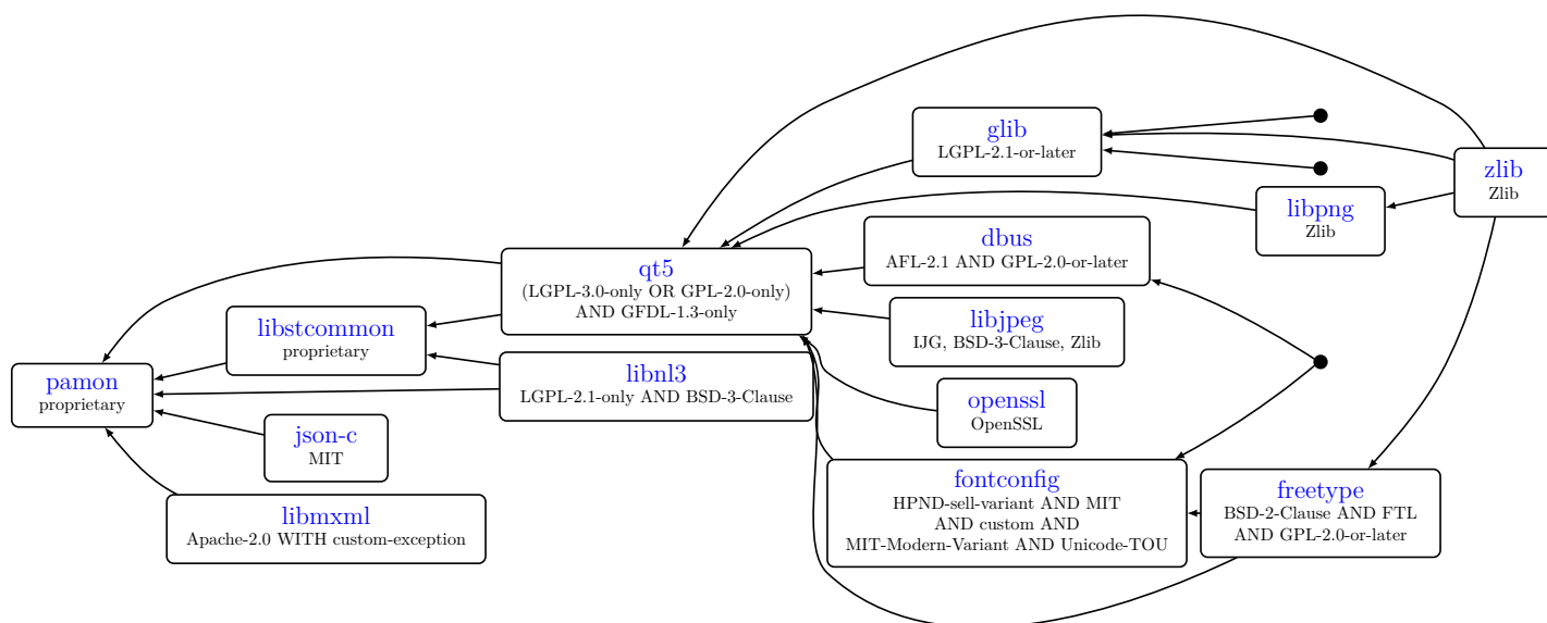
Figure 107.1: Dependency tree for pamon
