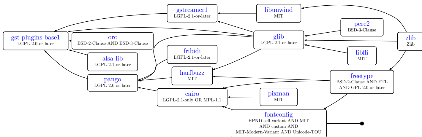
Figure 31.1: Dependency tree for gst-plugins-base1
