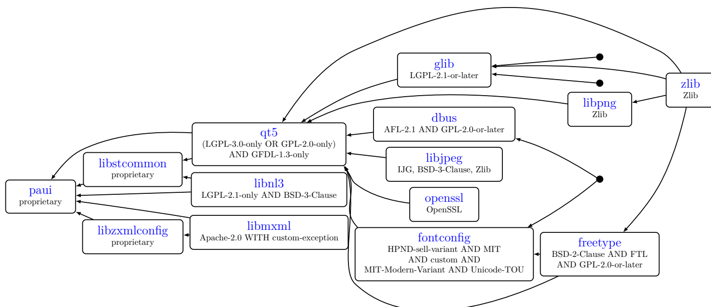
Figure 109.1: Dependency tree for paui
