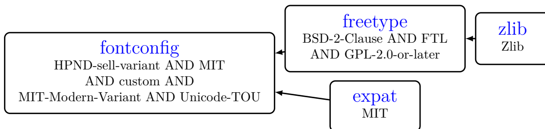
Figure 23.1: Dependency tree for fontconfig
